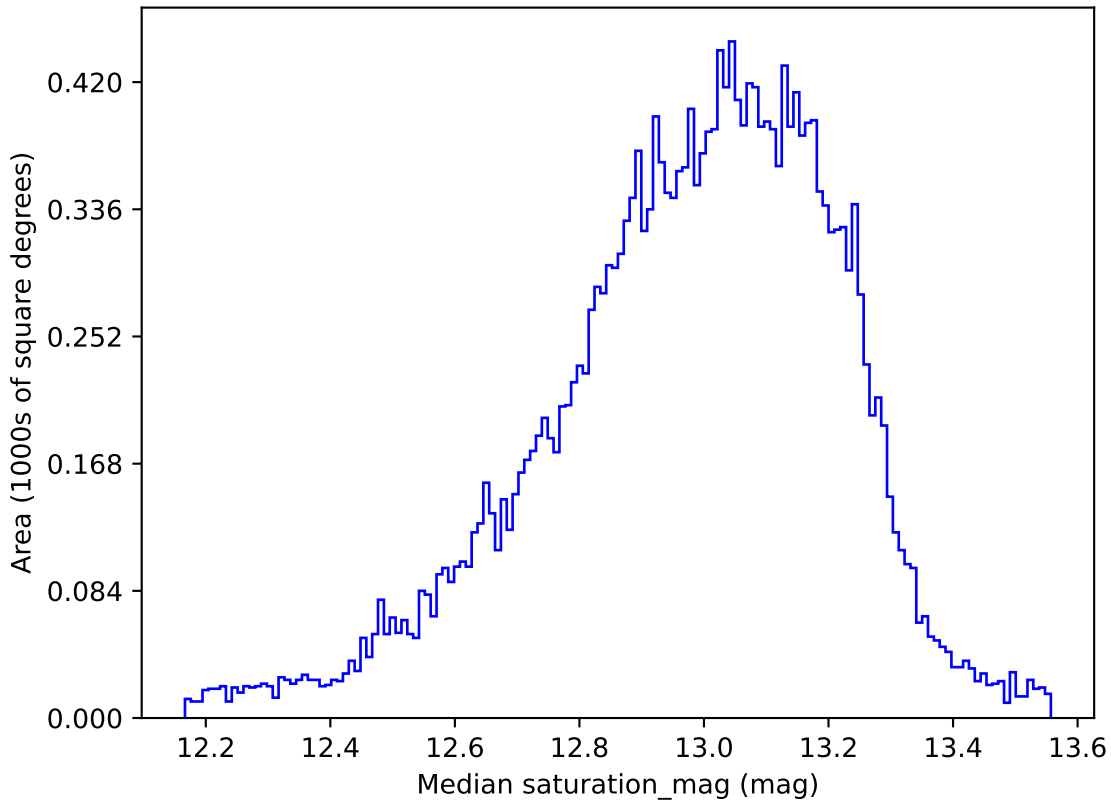
roll_pause_mjdp60_v3.4_10yrs All sky u band: Median saturation_mag
