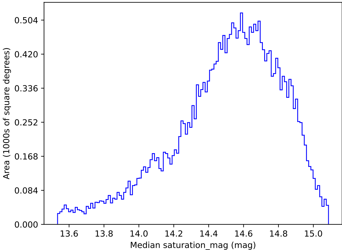
roll_pause_mjdp60_v3.4_10yrs All sky g band: Median saturation_mag
