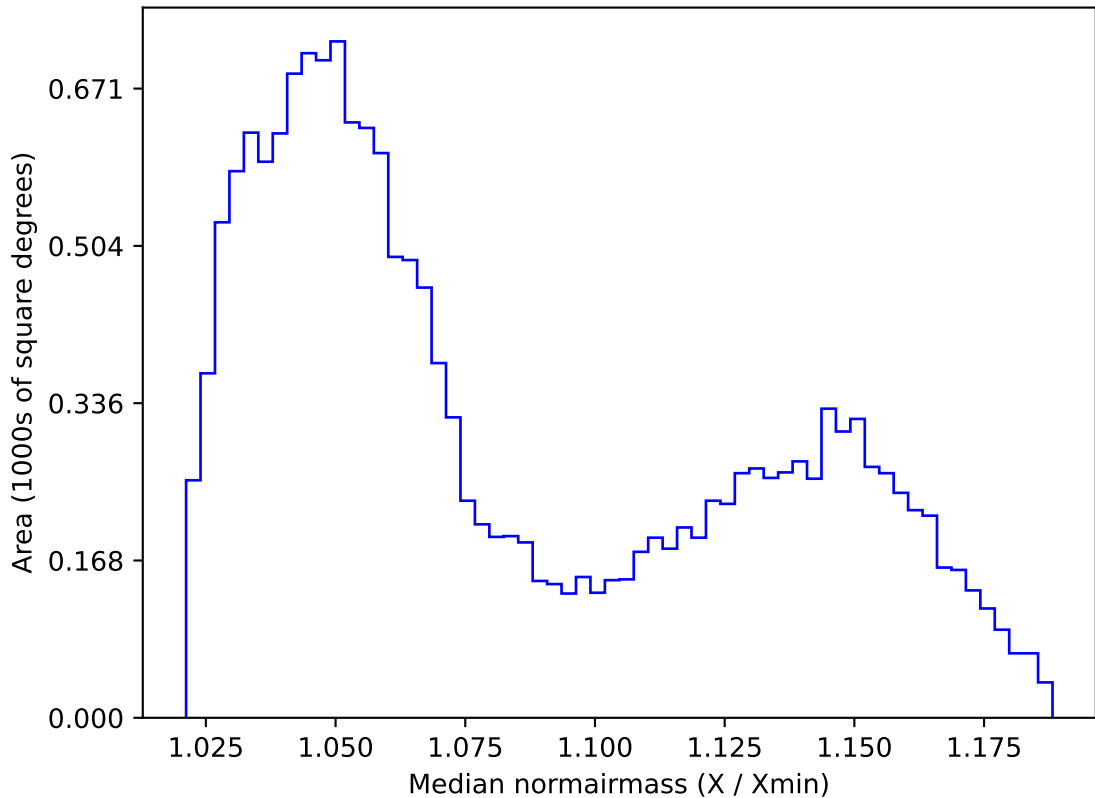
roll_pause_mjdp60_v3.4_10yrs WFD z band: Median normairmass
