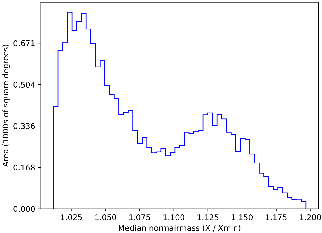
roll_pause_mjdp60_v3.4_10yrs WFD u band: Median normairmass
