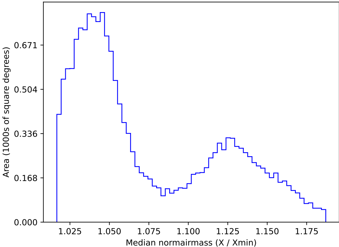
roll_pause_mjdp60_v3.4_10yrs WFD r band: Median normairmass
