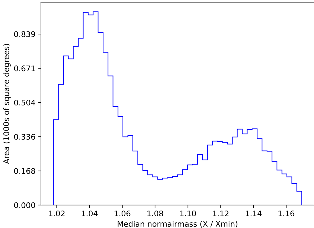
roll_pause_mjdp60_v3.4_10yrs WFD i band: Median normairmass
