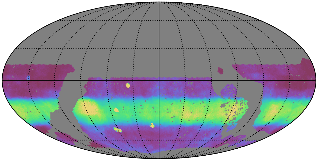
roll_pause_mjdp60_v3.4_10yrs WFD all bands: Median normairmass
