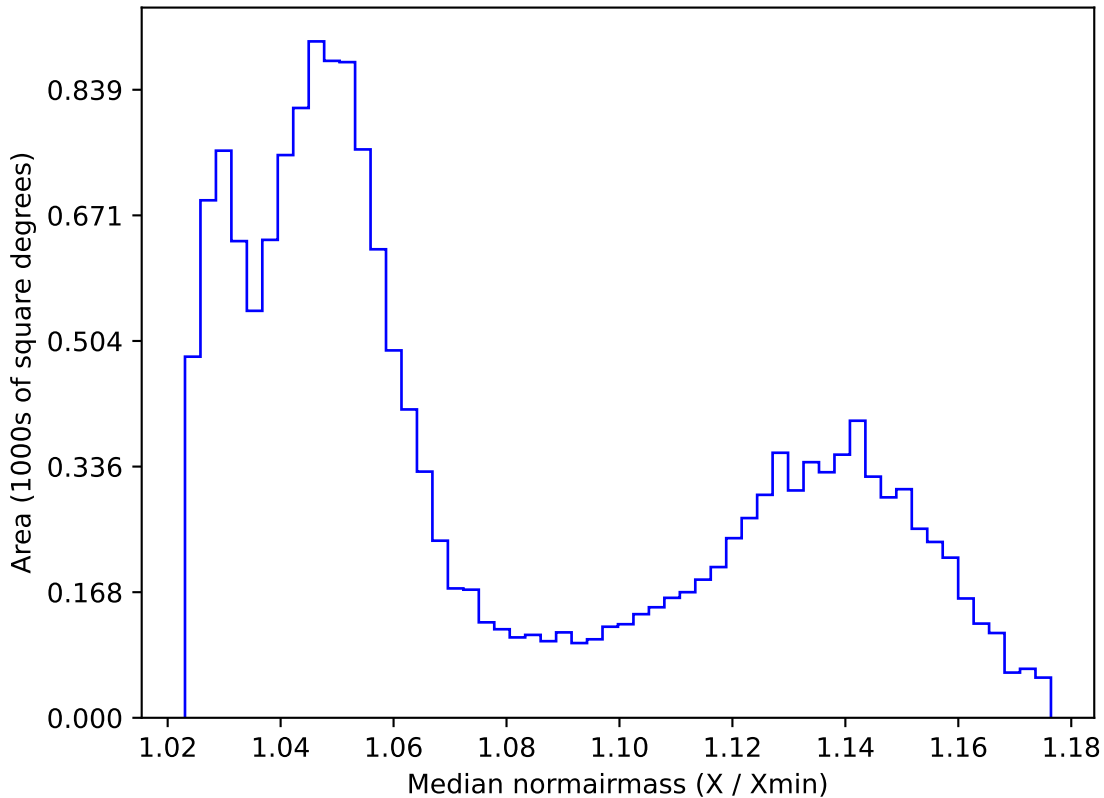
roll_pause_mjdp60_v3.4_10yrs WFD all bands: Median normairmass
