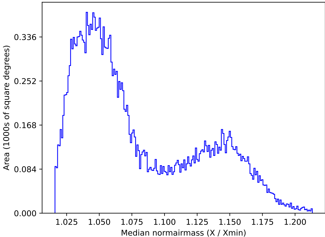
roll_pause_mjdp60_v3.4_10yrs All sky z band: Median normairmass
