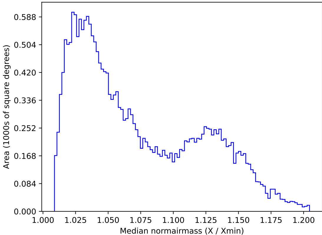
roll_pause_mjdp60_v3.4_10yrs All sky u band: Median normairmass
