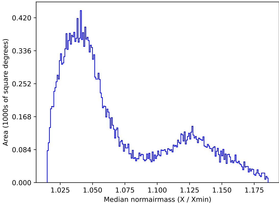
roll_pause_mjdp60_v3.4_10yrs All sky r band: Median normairmass
