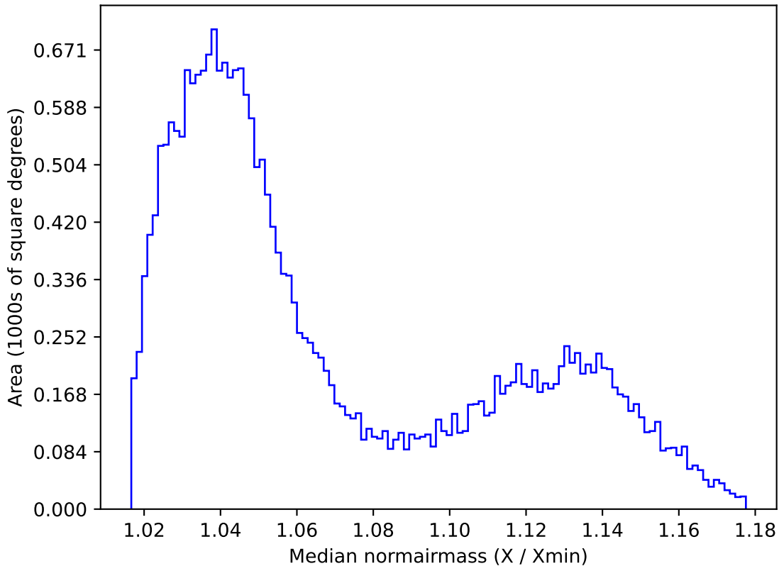
roll_pause_mjdp60_v3.4_10yrs All sky i band: Median normairmass
