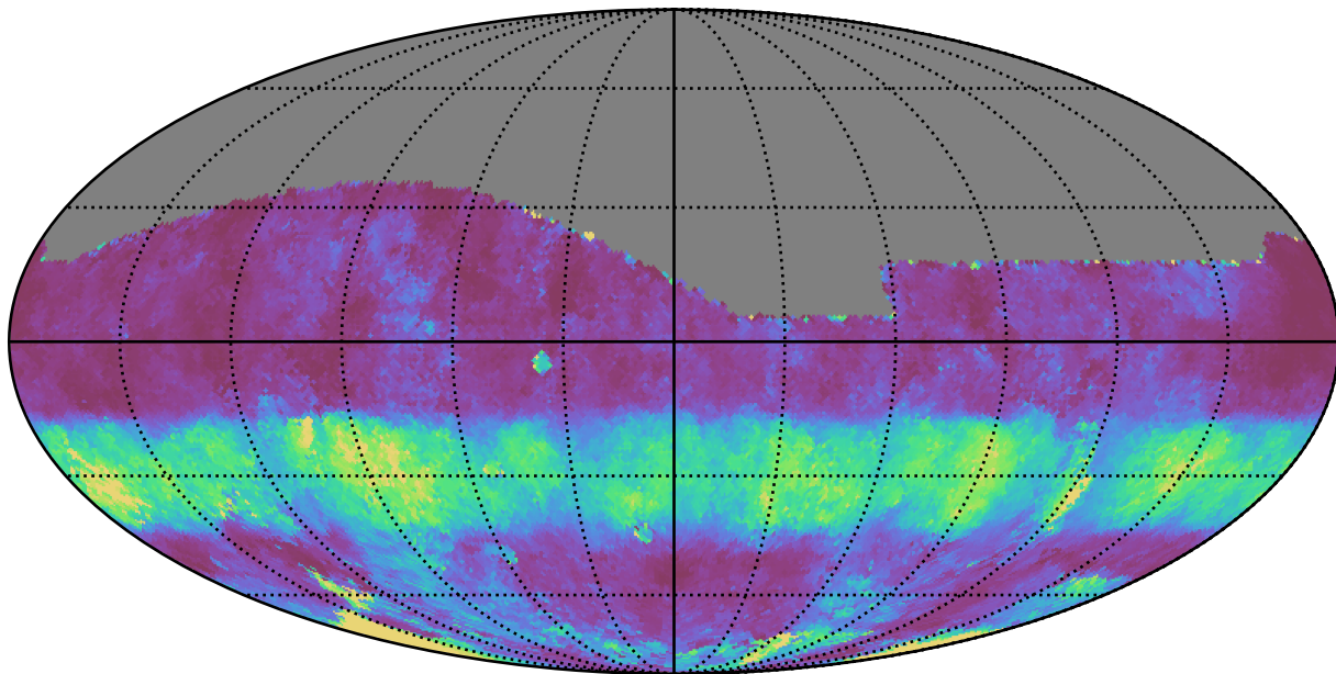
roll_pause_mjdp60_v3.4_10yrs All sky g band: Median normairmass
