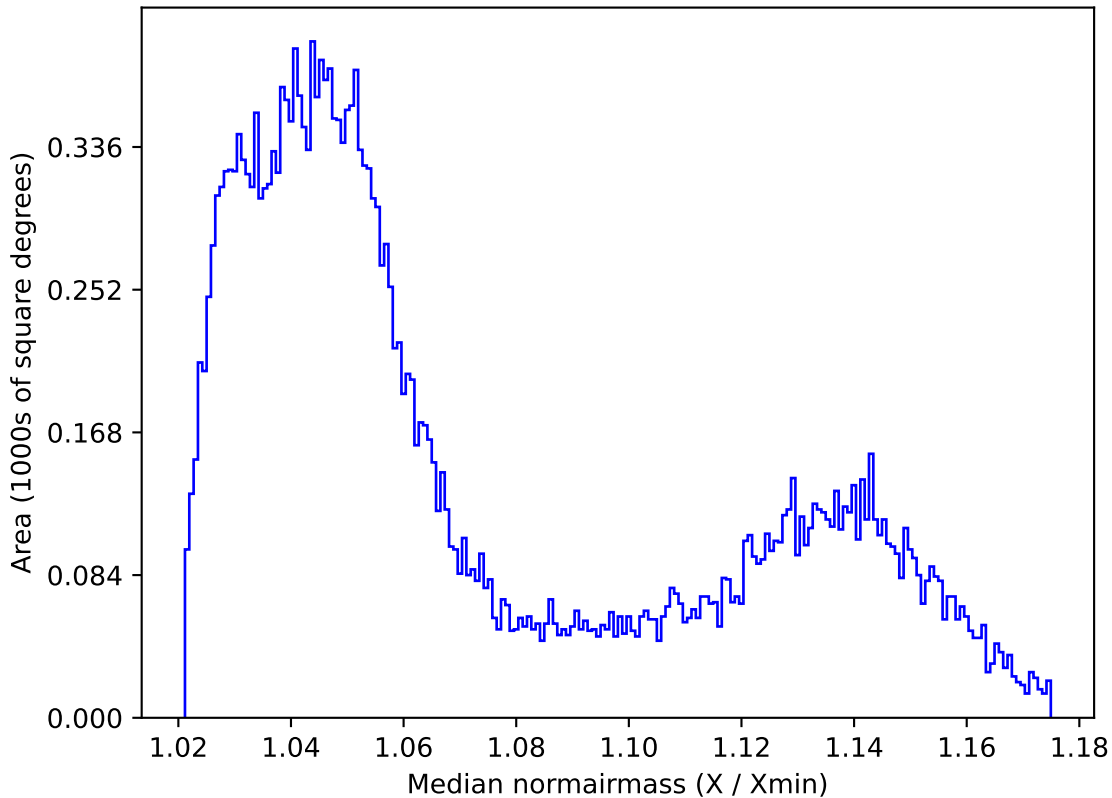
roll_pause_mjdp60_v3.4_10yrs All sky all bands: Median normairmass
