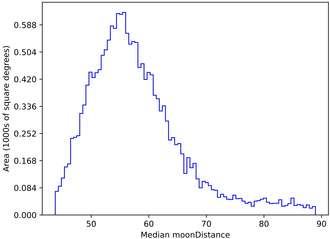
roll_pause_mjdp60_v3.4_10yrs WFD y band: Median moonDistance
