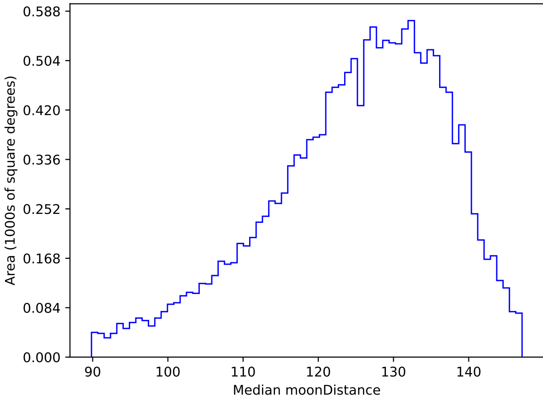
roll_pause_mjdp60_v3.4_10yrs WFD u band: Median moonDistance
