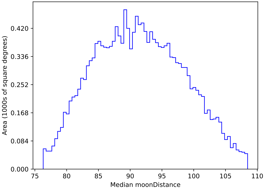
roll_pause_mjdp60_v3.4_10yrs WFD i band: Median moonDistance
