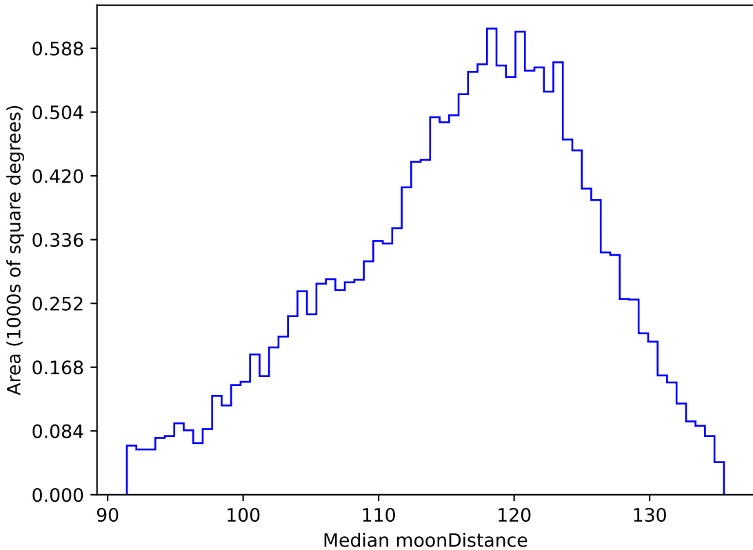
roll_pause_mjdp60_v3.4_10yrs WFD g band: Median moonDistance
