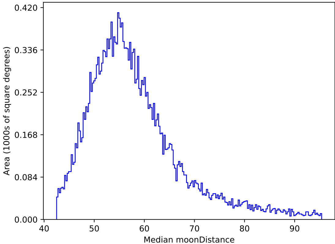
roll_pause_mjdp60_v3.4_10yrs All sky y band: Median moonDistance
