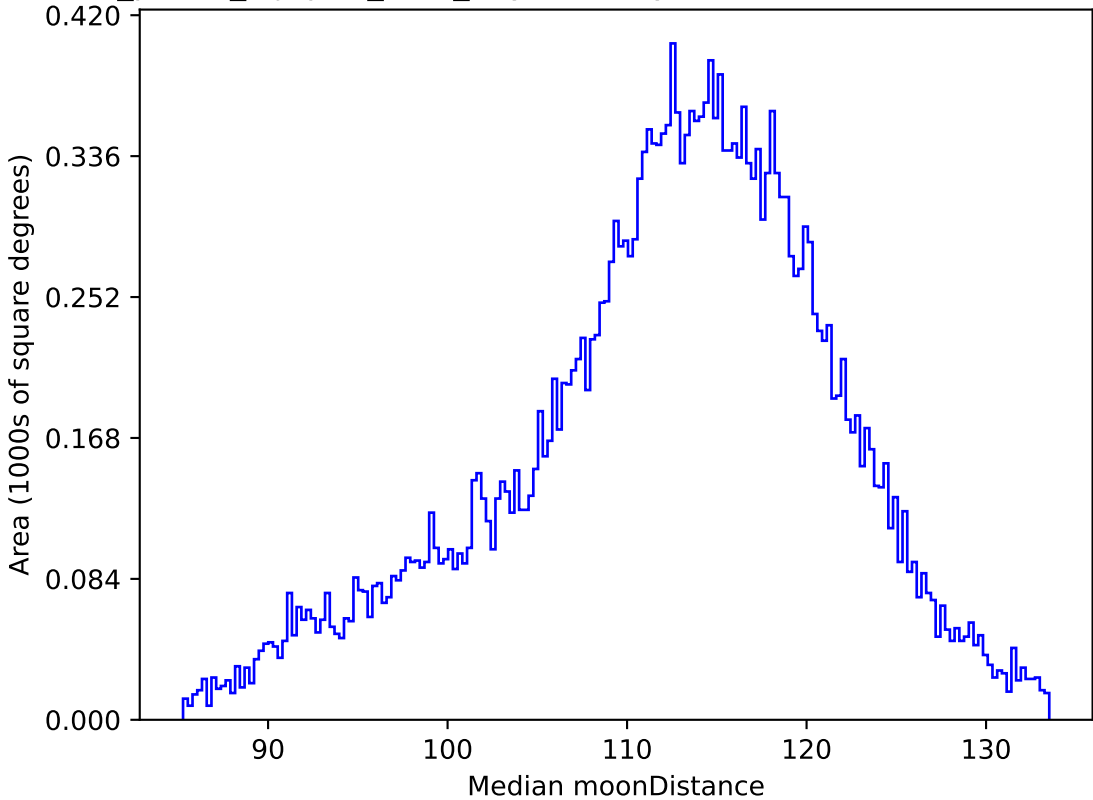
roll_pause_mjdp60_v3.4_10yrs All sky r band: Median moonDistance
