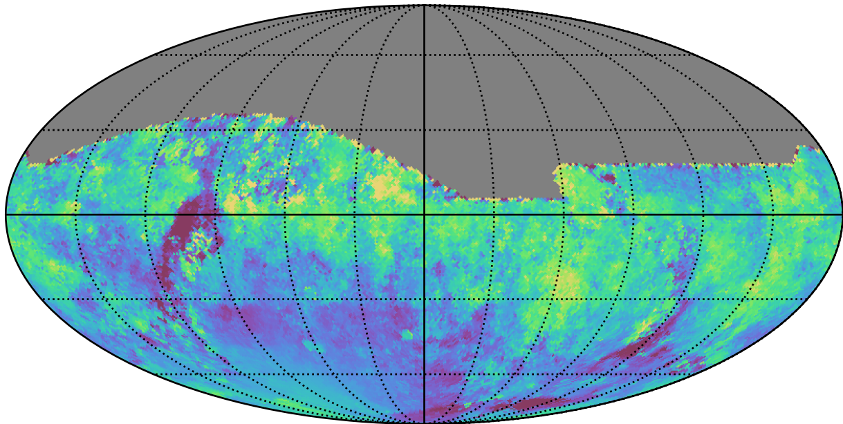
roll_pause_mjdp60_v3.4_10yrs All sky i band: Median moonDistance
