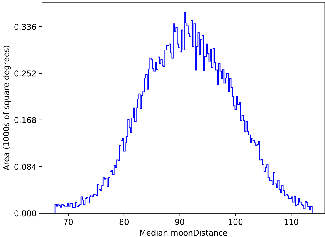
roll_pause_mjdp60_v3.4_10yrs All sky i band: Median moonDistance
