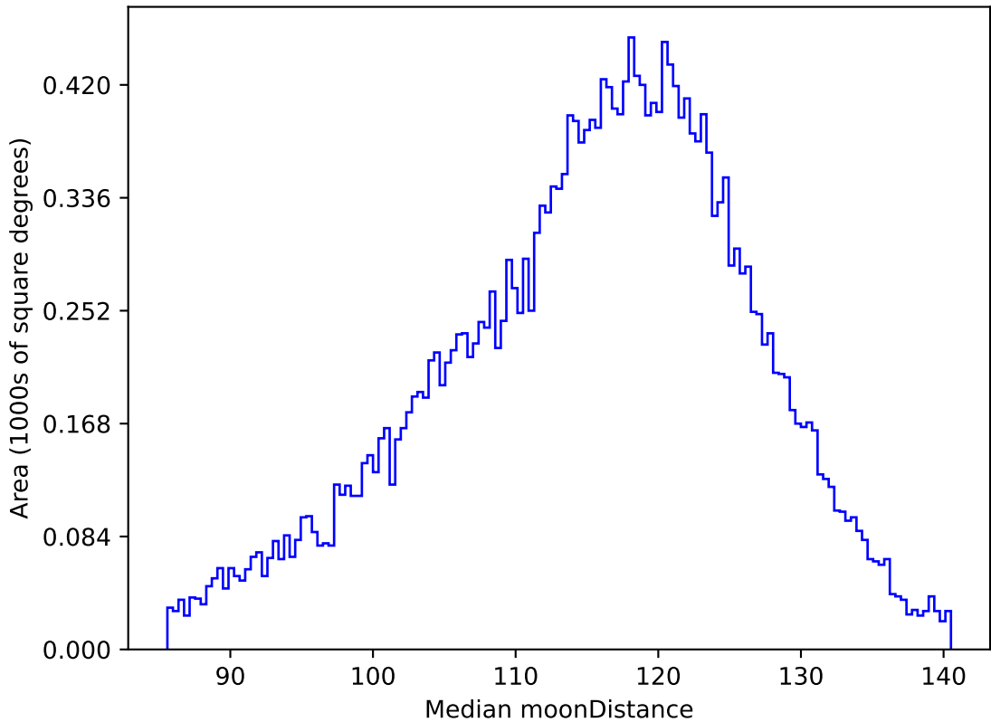
roll_pause_mjdp60_v3.4_10yrs All sky g band: Median moonDistance
