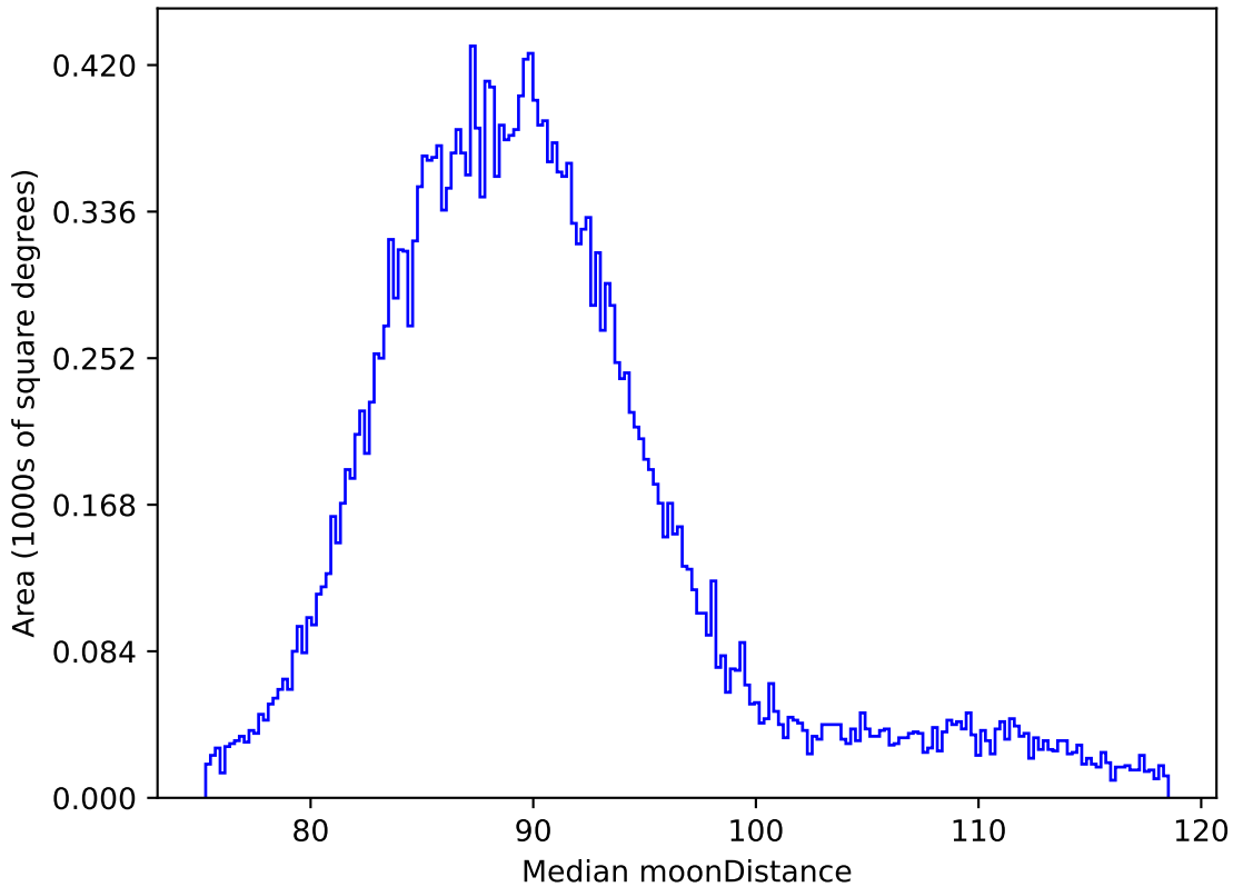
roll_pause_mjdp60_v3.4_10yrs All sky all bands: Median moonDistance
