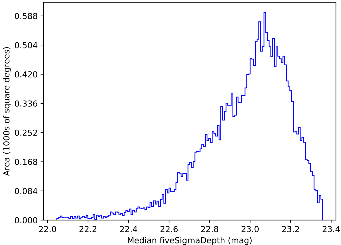
roll_pause_mjdp60_v3.4_10yrs Yr 1 z band: Median fiveSigmaDepth
