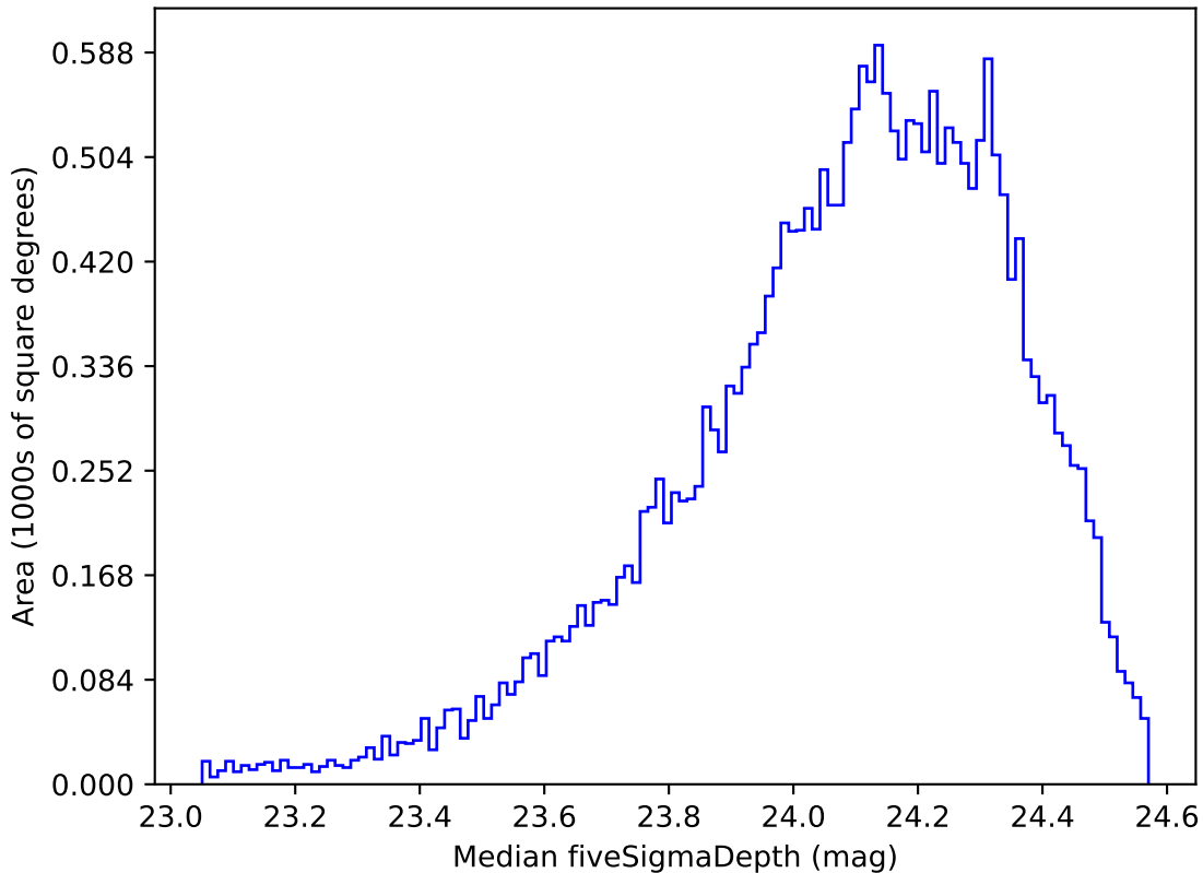
roll_pause_mjdp60_v3.4_10yrs Yr 1 r band: Median fiveSigmaDepth
