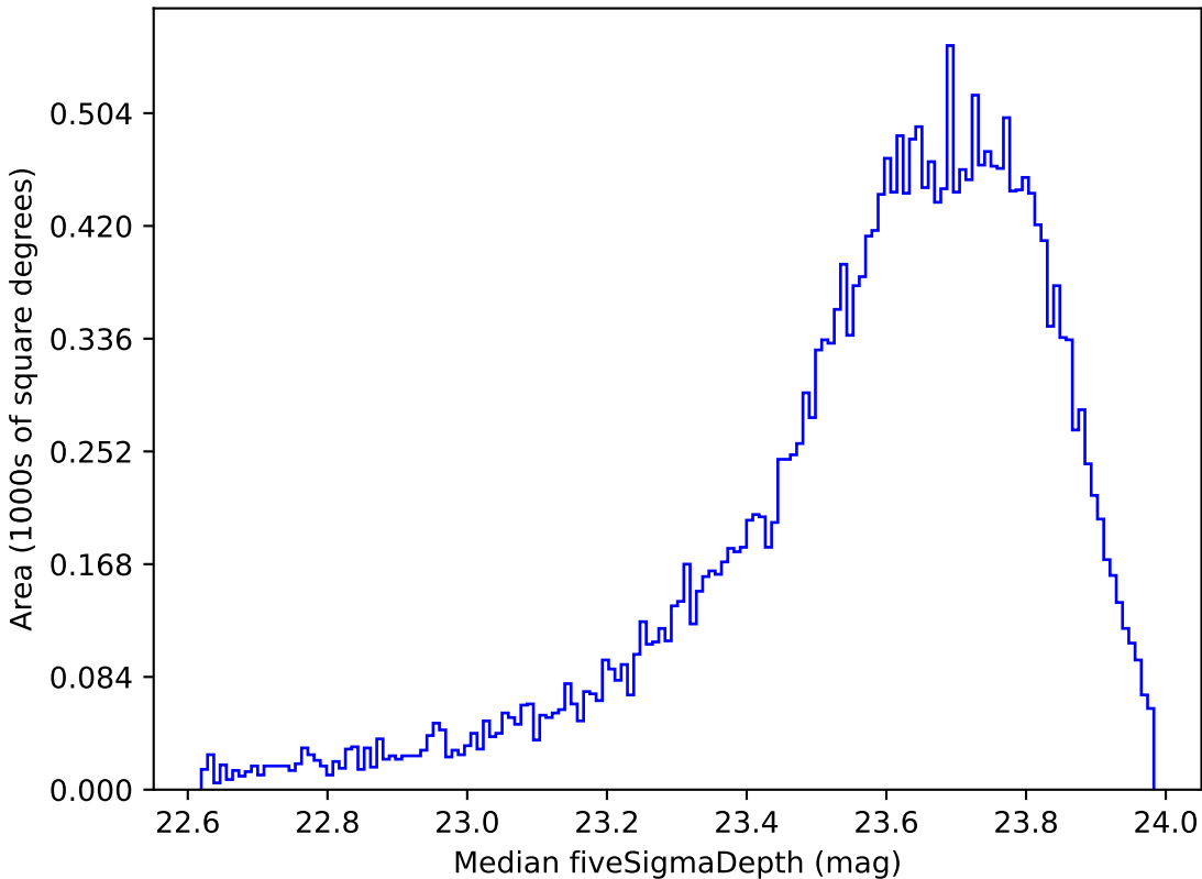
roll_pause_mjdp60_v3.4_10yrs Yr 1 i band: Median fiveSigmaDepth
