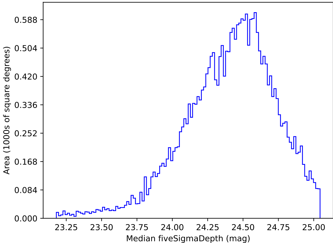
roll_pause_mjdp60_v3.4_10yrs Yr 1 g band: Median fiveSigmaDepth
