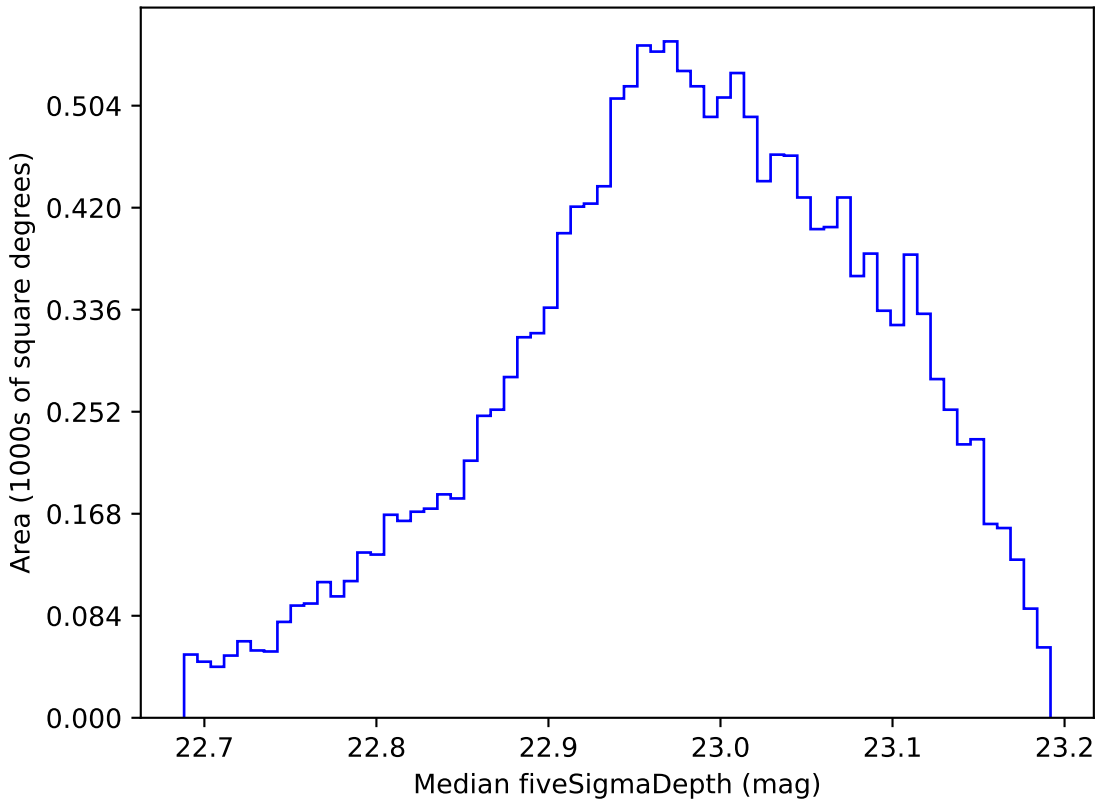
roll_pause_mjdp60_v3.4_10yrs WFD z band: Median fiveSigmaDepth
