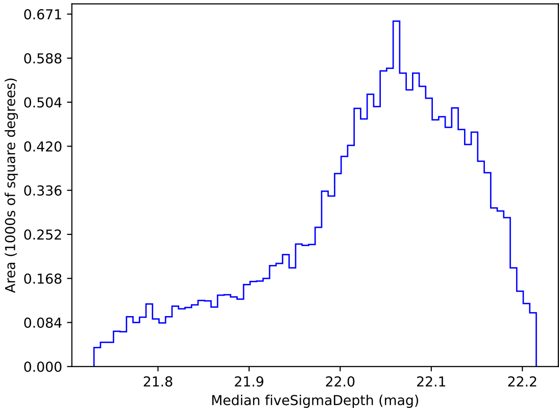
roll_pause_mjdp60_v3.4_10yrs WFD y band: Median fiveSigmaDepth
