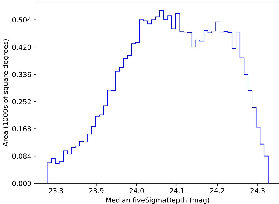
roll_pause_mjdp60_v3.4_10yrs WFD r band: Median fiveSigmaDepth
