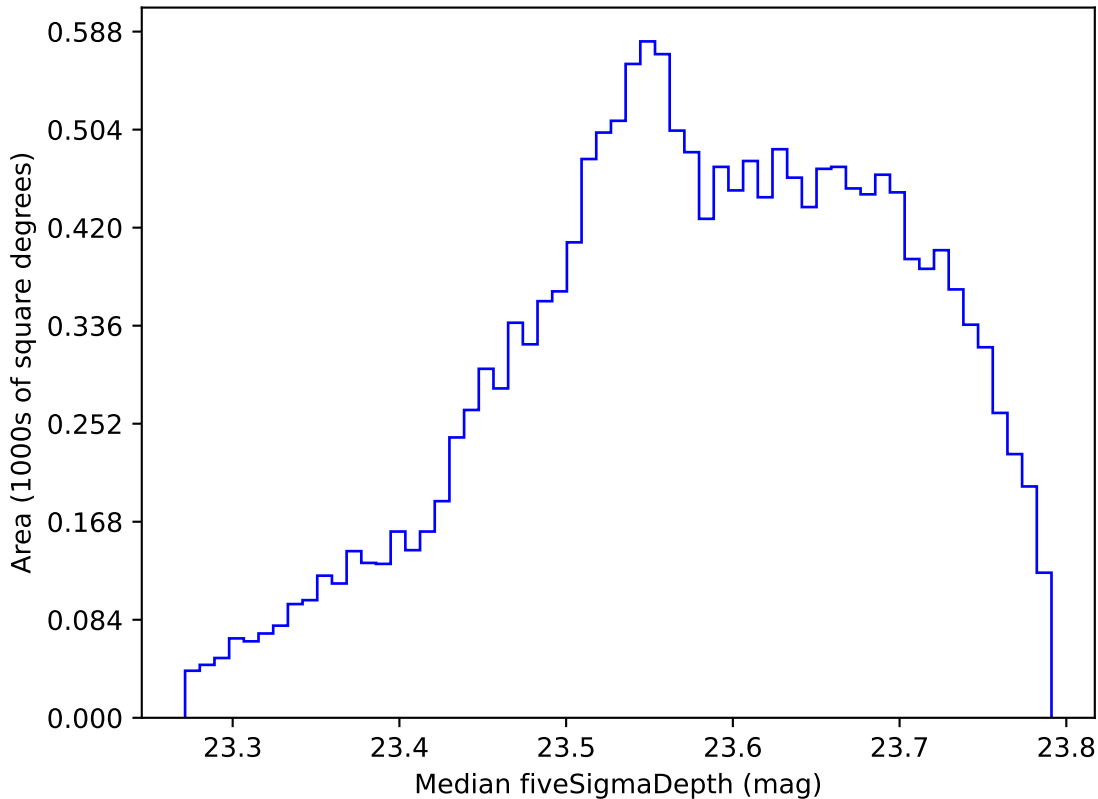
roll_pause_mjdp60_v3.4_10yrs WFD i band: Median fiveSigmaDepth
