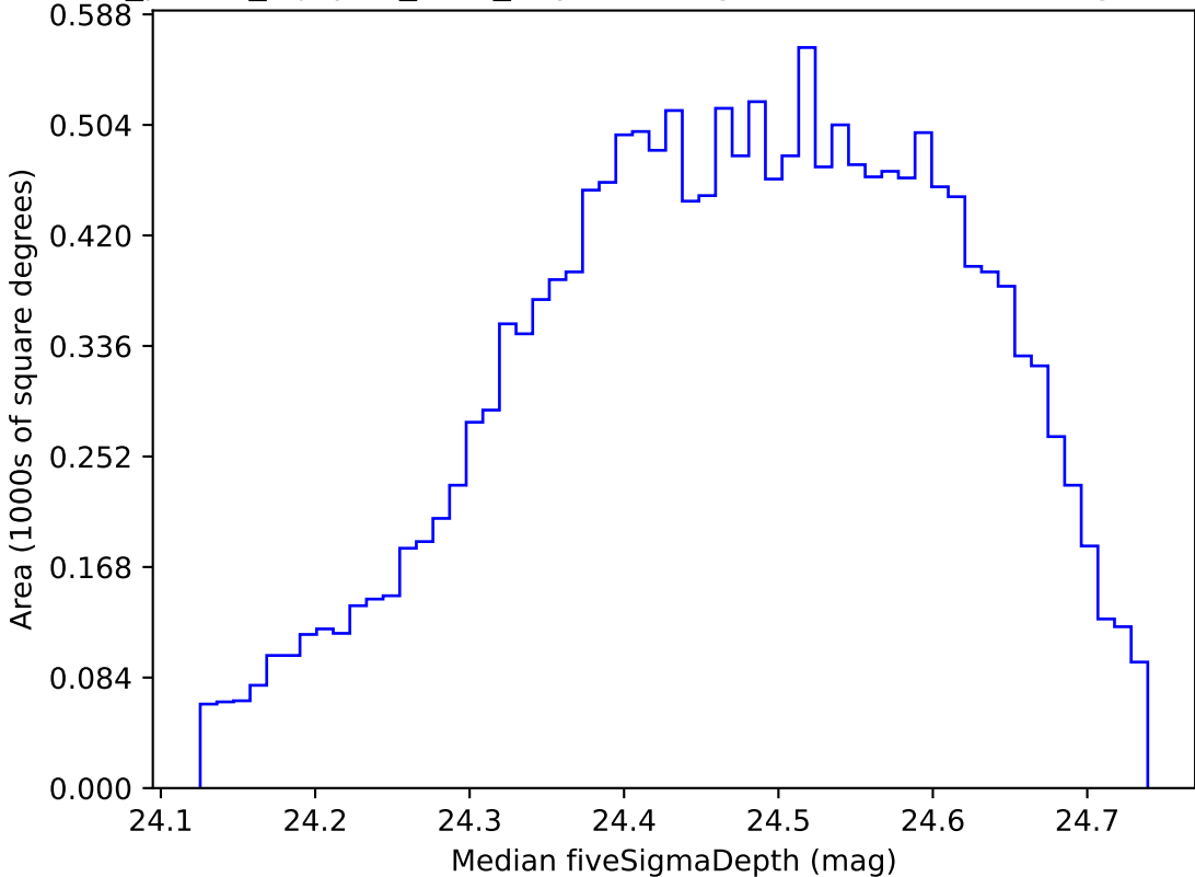
roll_pause_mjdp60_v3.4_10yrs WFD g band: Median fiveSigmaDepth
