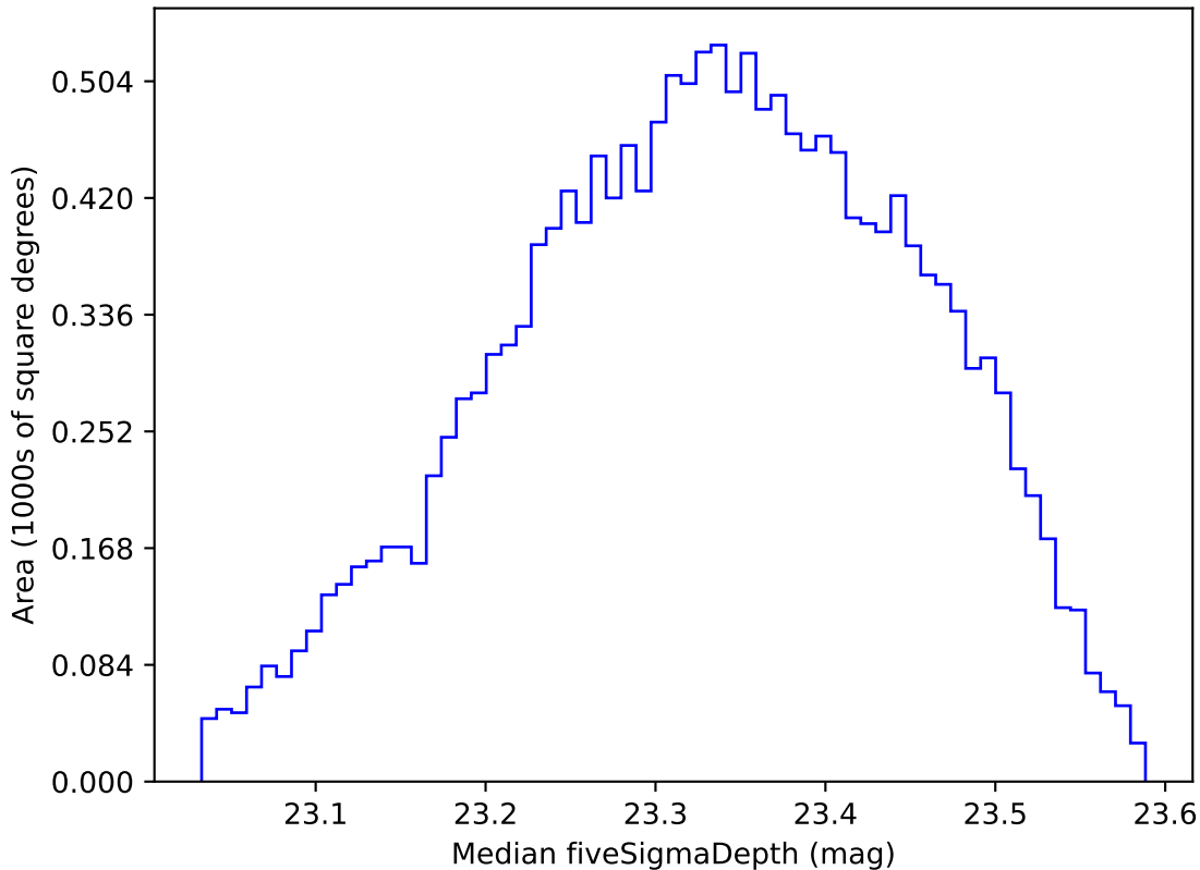
roll_pause_mjdp60_v3.4_10yrs WFD all bands: Median fiveSigmaDepth
