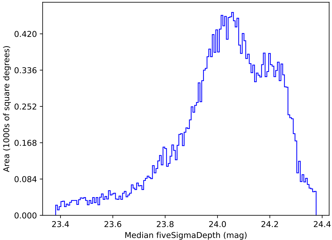
roll_pause_mjdp60_v3.4_10yrs All sky r band: Median fiveSigmaDepth
