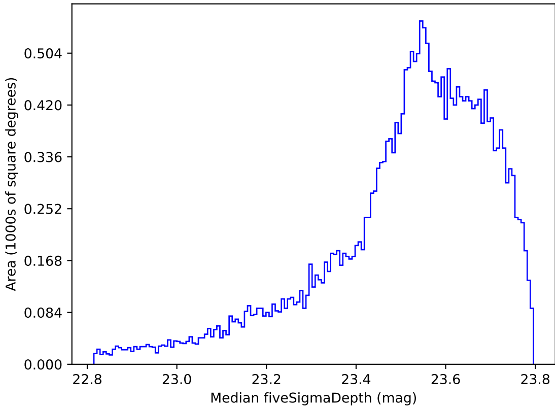
roll_pause_mjdp60_v3.4_10yrs All sky i band: Median fiveSigmaDepth
