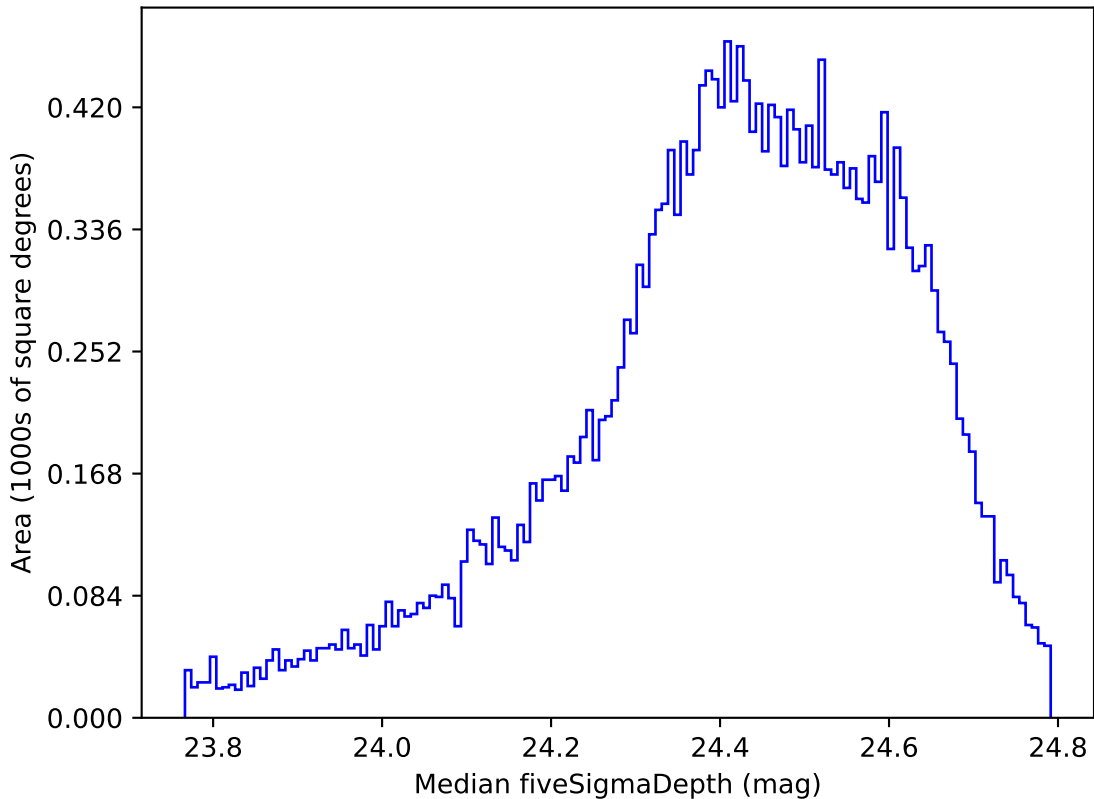
roll_pause_mjdp60_v3.4_10yrs All sky g band: Median fiveSigmaDepth
