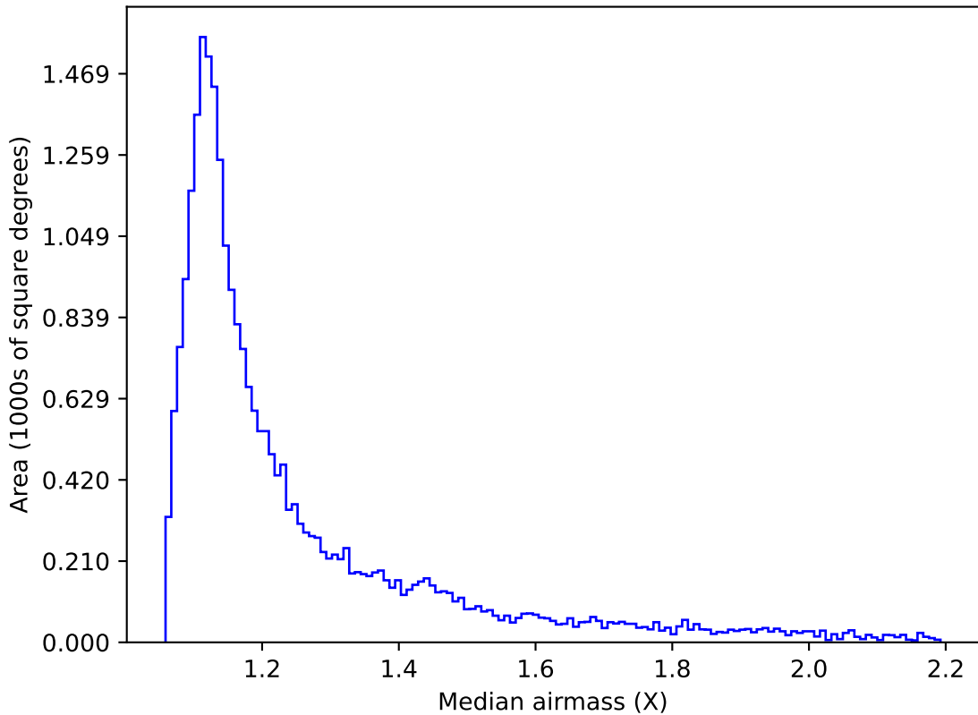
roll_pause_mjdp60_v3.4_10yrs Yr 1 z band: Median airmass
