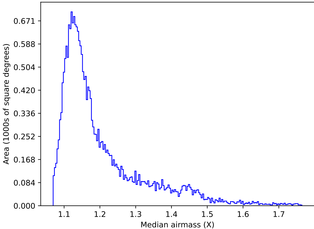
roll_pause_mjdp60_v3.4_10yrs Yr 1 y band: Median airmass
