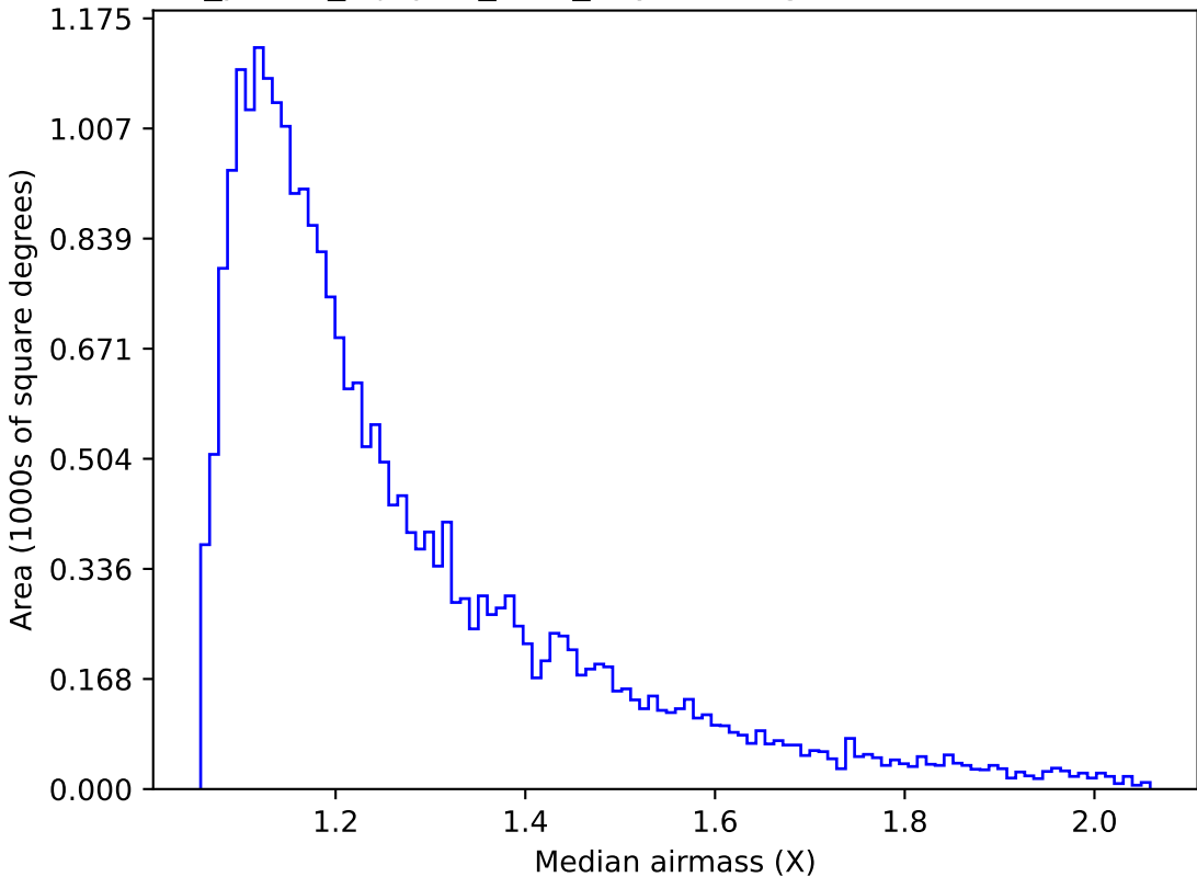
roll_pause_mjdp60_v3.4_10yrs Yr 1 g band: Median airmass
