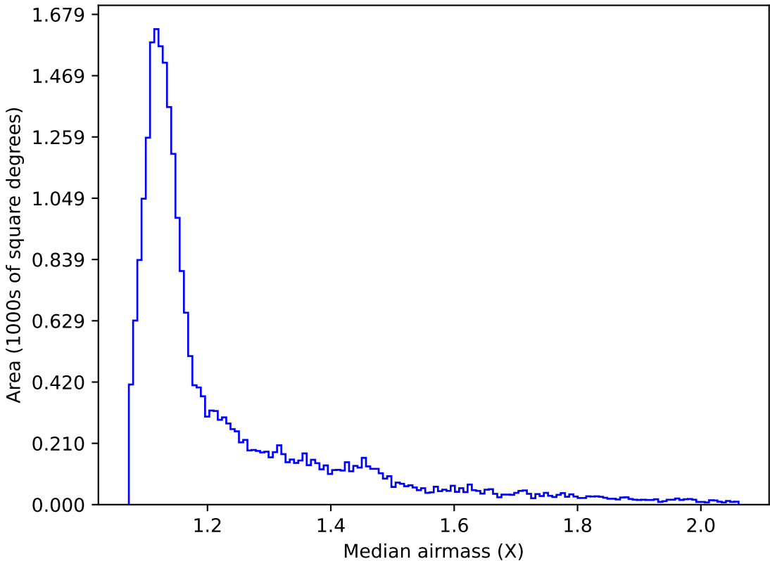
roll_pause_mjdp60_v3.4_10yrs Yr 1 all bands: Median airmass
