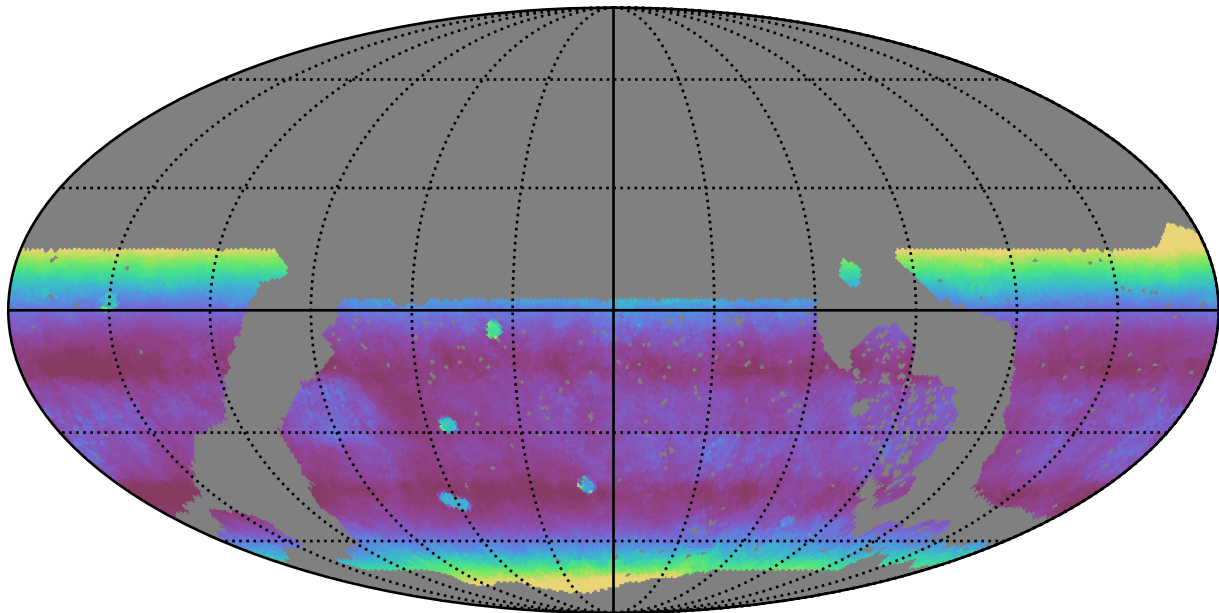
roll_pause_mjdp60_v3.4_10yrs WFD z band: Median airmass
