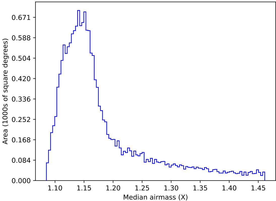
roll_pause_mjdp60_v3.4_10yrs WFD z band: Median airmass
