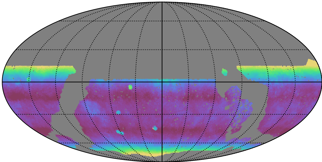
roll_pause_mjdp60_v3.4_10yrs WFD y band: Median airmass
