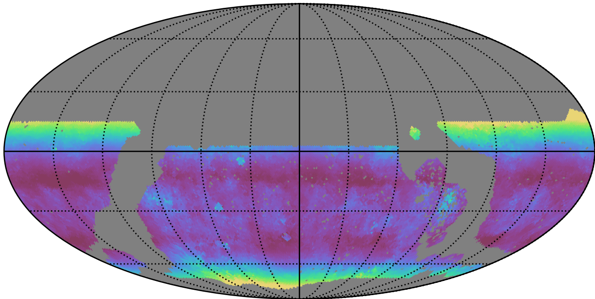
roll_pause_mjdp60_v3.4_10yrs WFD u band: Median airmass
