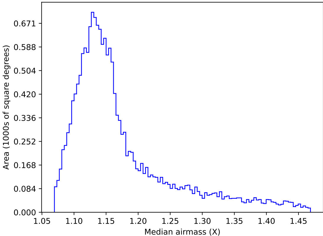
roll_pause_mjdp60_v3.4_10yrs WFD u band: Median airmass
