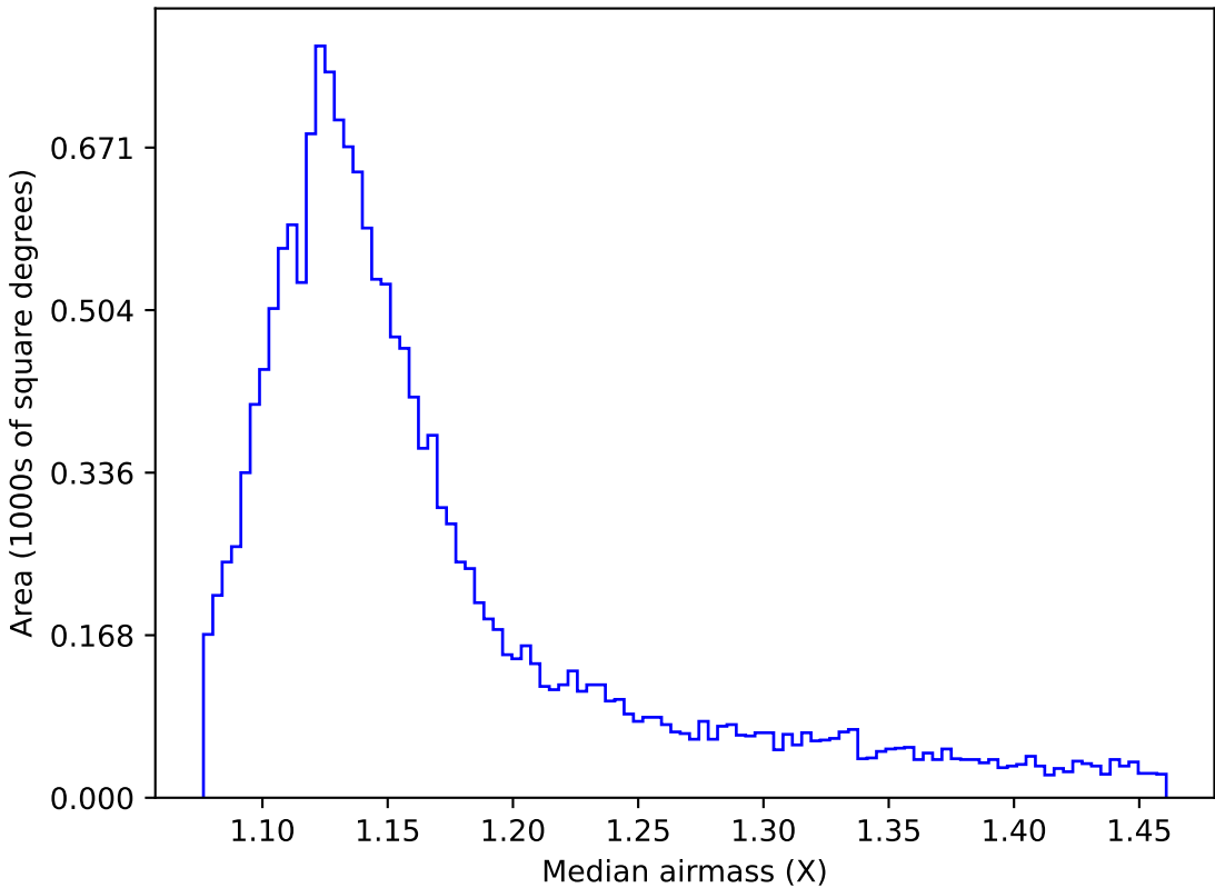
roll_pause_mjdp60_v3.4_10yrs WFD r band: Median airmass
