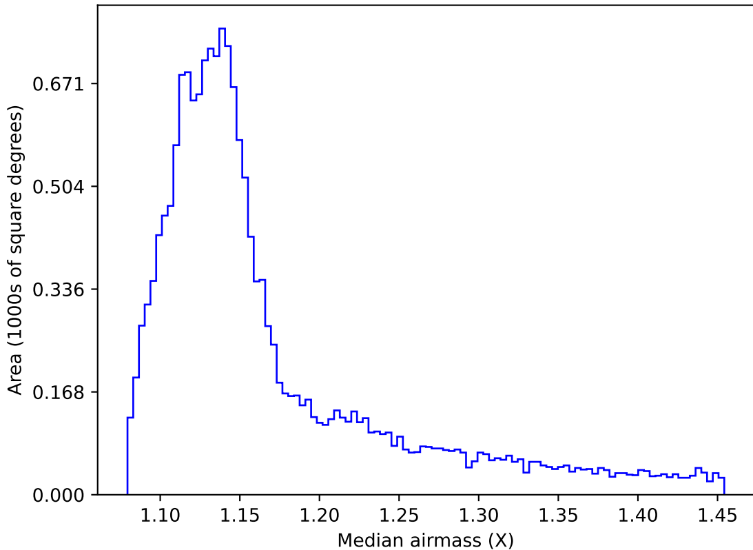
roll_pause_mjdp60_v3.4_10yrs WFD i band: Median airmass
