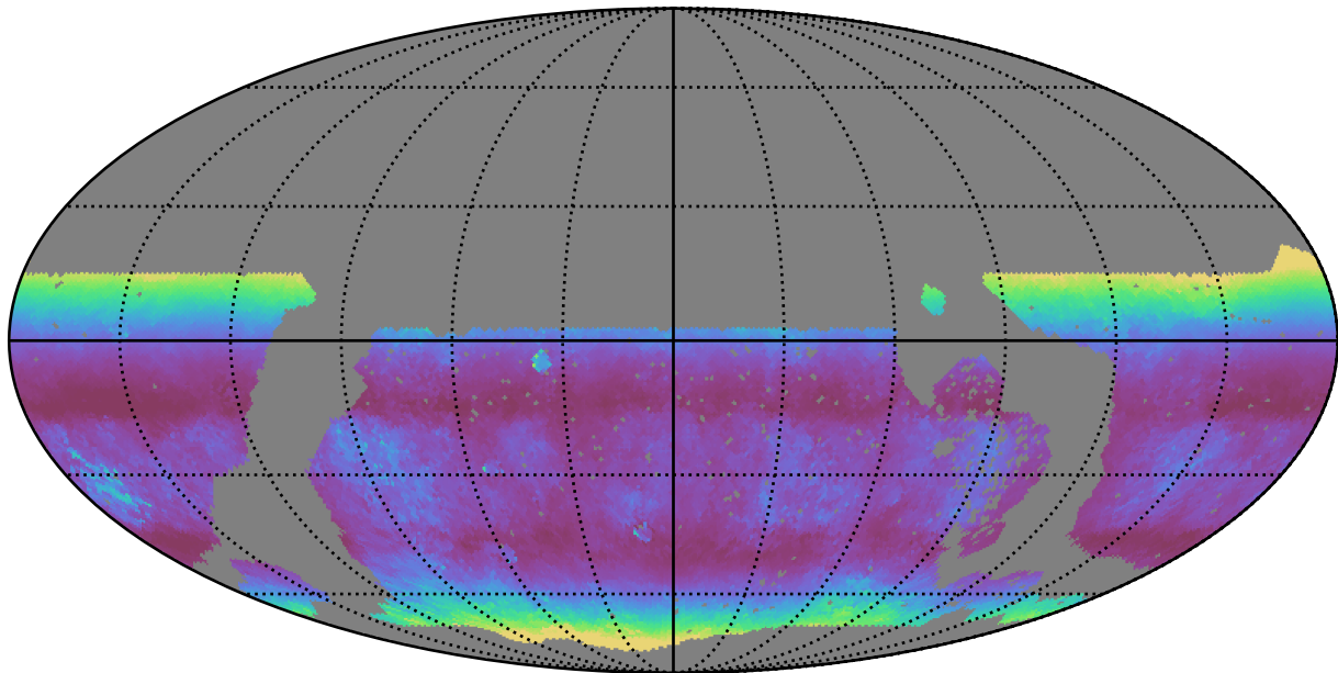
roll_pause_mjdp60_v3.4_10yrs WFD g band: Median airmass
