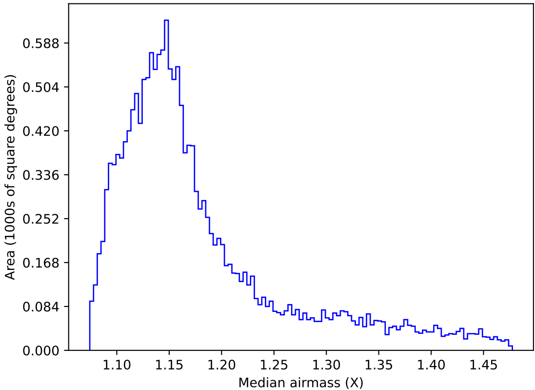
roll_pause_mjdp60_v3.4_10yrs WFD g band: Median airmass
